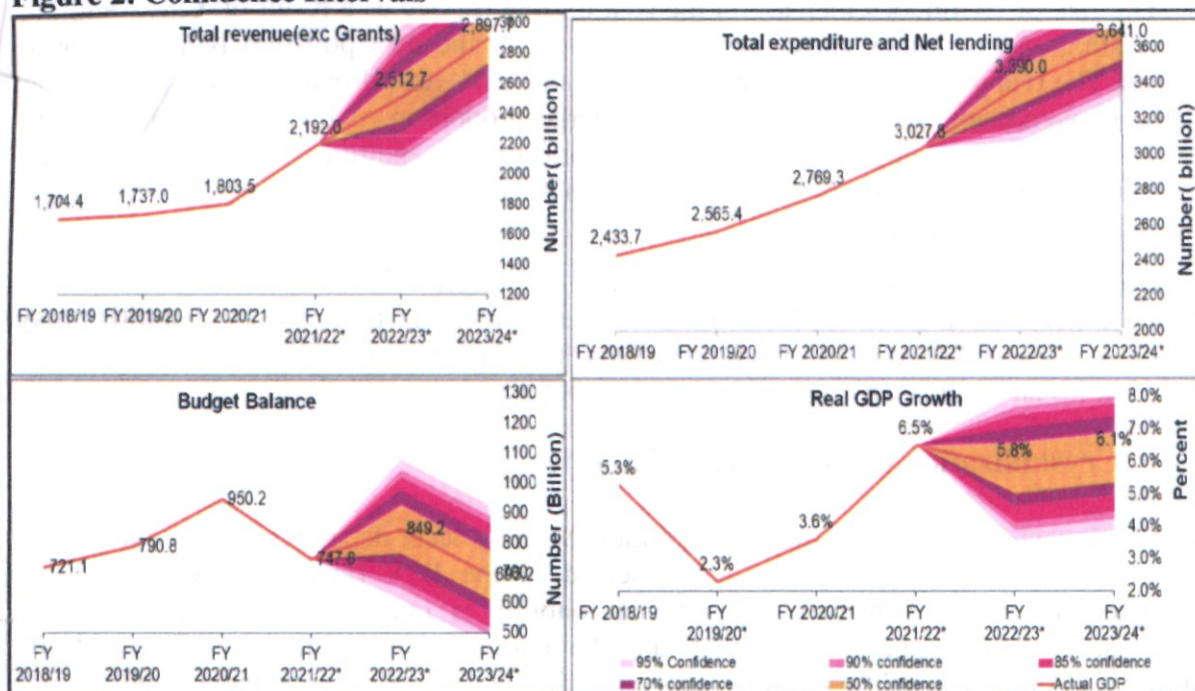
Figure 2: Confidence Intervals
